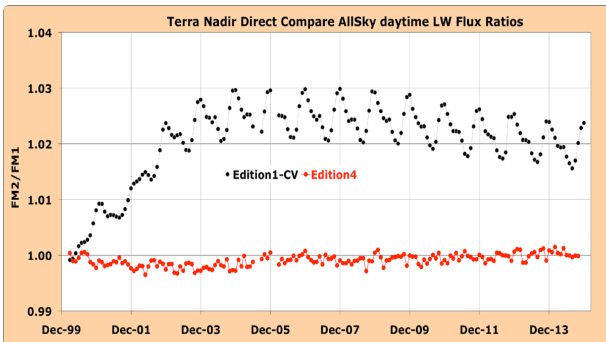
Figure 2-2. Terra nadir direct compare ratios for LW day time all sky fluxes.
